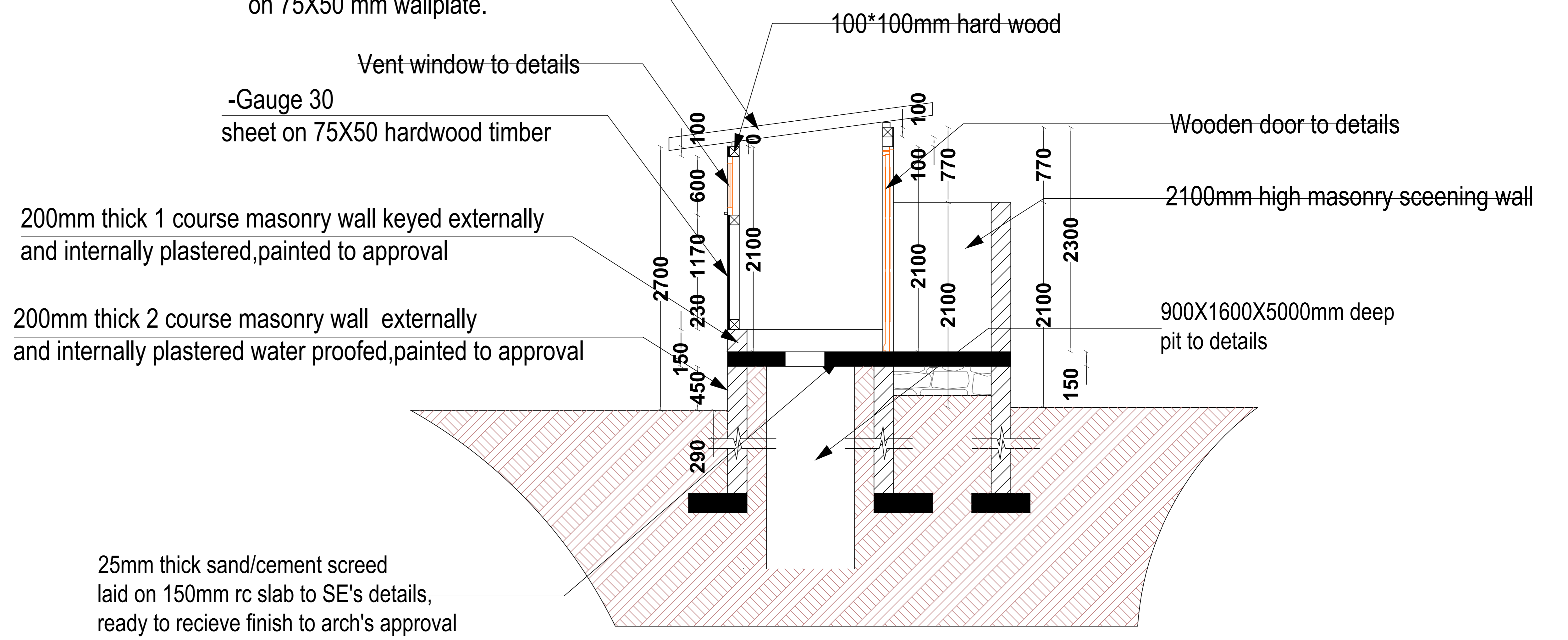
SECTION X-X
